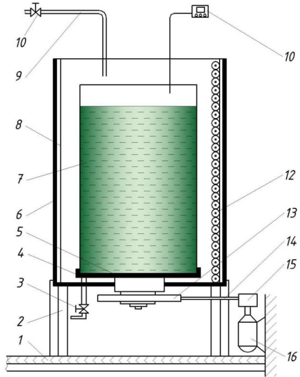
Fig.1. Bioreactor for green algae growth. 1-Floor; 2-stand; 3-chlorella drain tap; 4-reservoir stand; 5-frame; 6-main body; 7-glass container; 8-foil; 9-pipe; 10-screw adapter; 11-temperature sensor; 12-sodium lamp; 13,15-pulley; 14-belt; 16-mini electric motor
