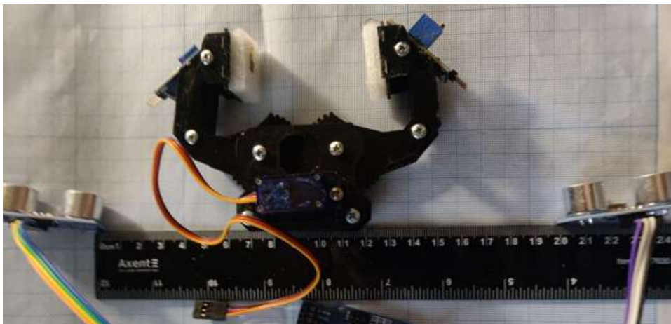
Figure 2: General prototype for research using the triangulation method to determine distance to an object
