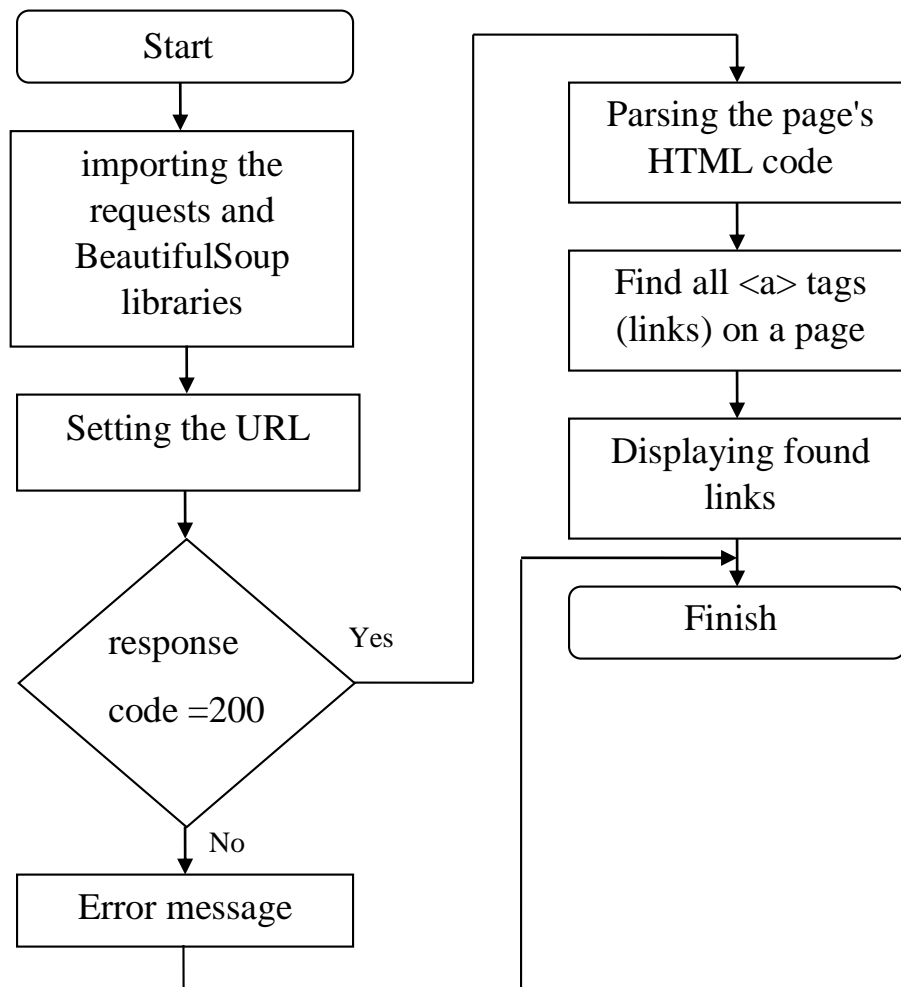
Figure 1: The Web Site https://tapr.nure.ua/en/ parsing program algorithm
