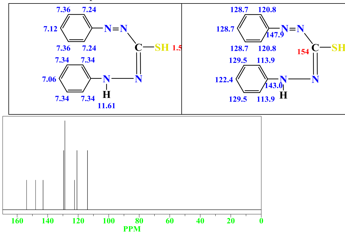
5-rasm. Ditiononning 13C spektri
