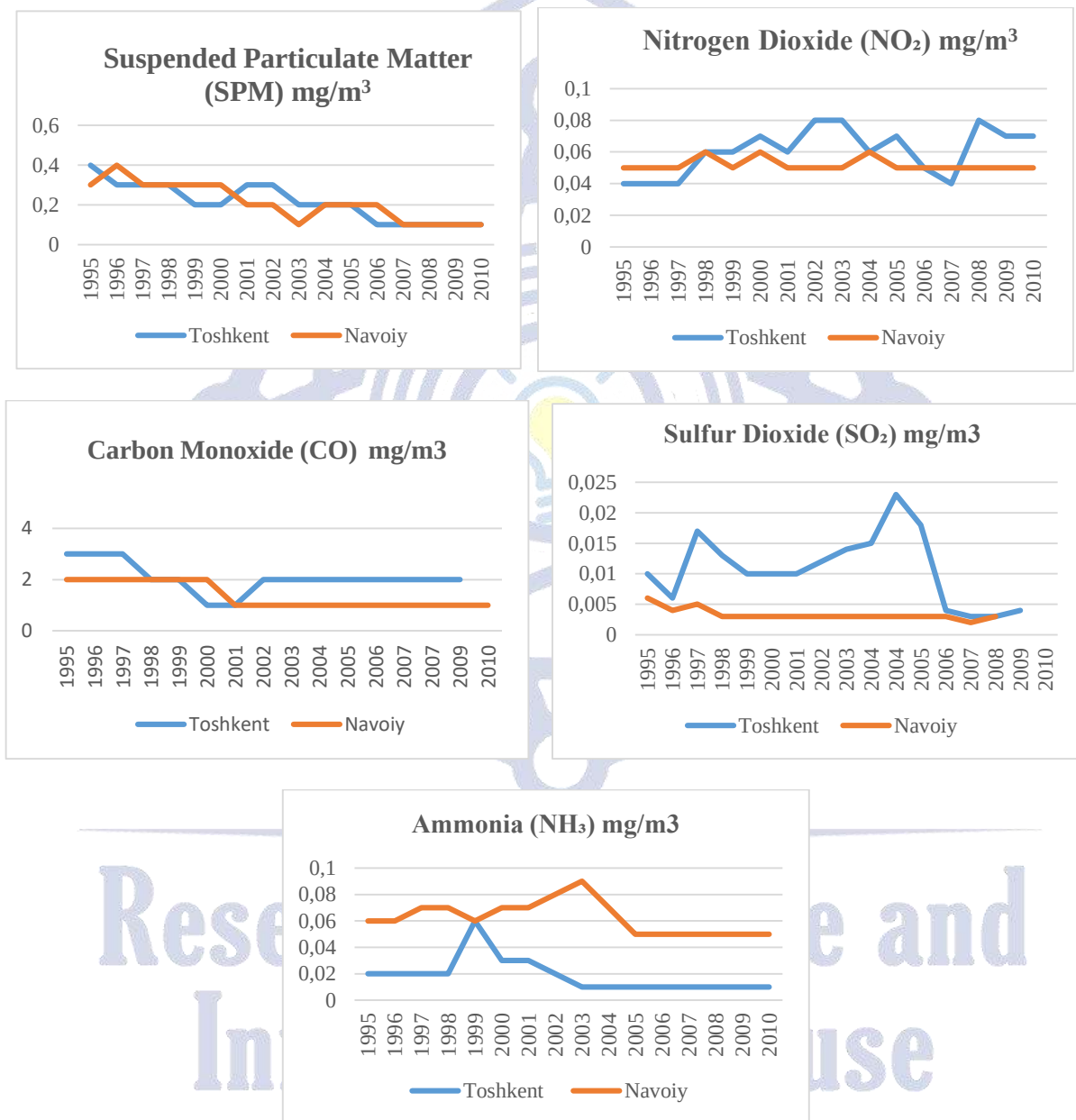
Figure 1. Fluctuation graph of atmospheric pollutant gases in Tashkent and Navoiy cities during 1995–2010.
