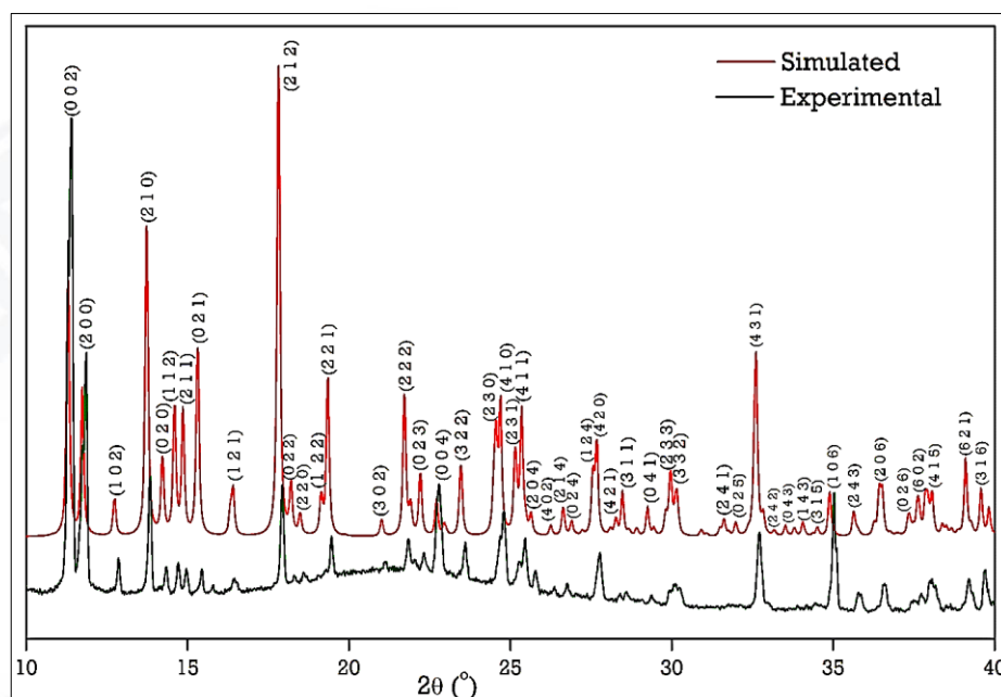
Figure 1. Comparison of simulated and experimental PXRD patterns of the one-dimensional cadmium(II) isonicotinate coordination polymer [\text{Cd}(\mu\text{-INA})(\text{NO}_3)(\text{H}_2\text{O})_2]_n .
