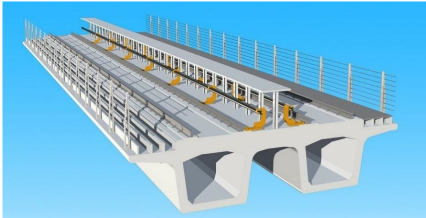
In order to reduce weight, various shapes of cavities (round, oval or rectangular) are created in monolithic intermediate devices. In terms of their working characteristics, such structures are close to multi-contour box intermediate devices (Figure 2).
